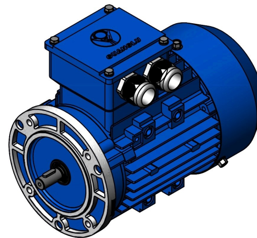
GL-63-B14B Mounting diagram
